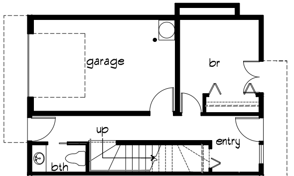
1st floor
